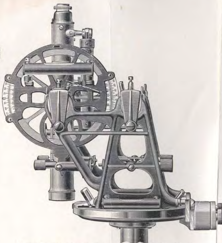
Instrument with Telescope, Vertical Circle, etc., in the Excentric Bearings. Counterpoise attached.
