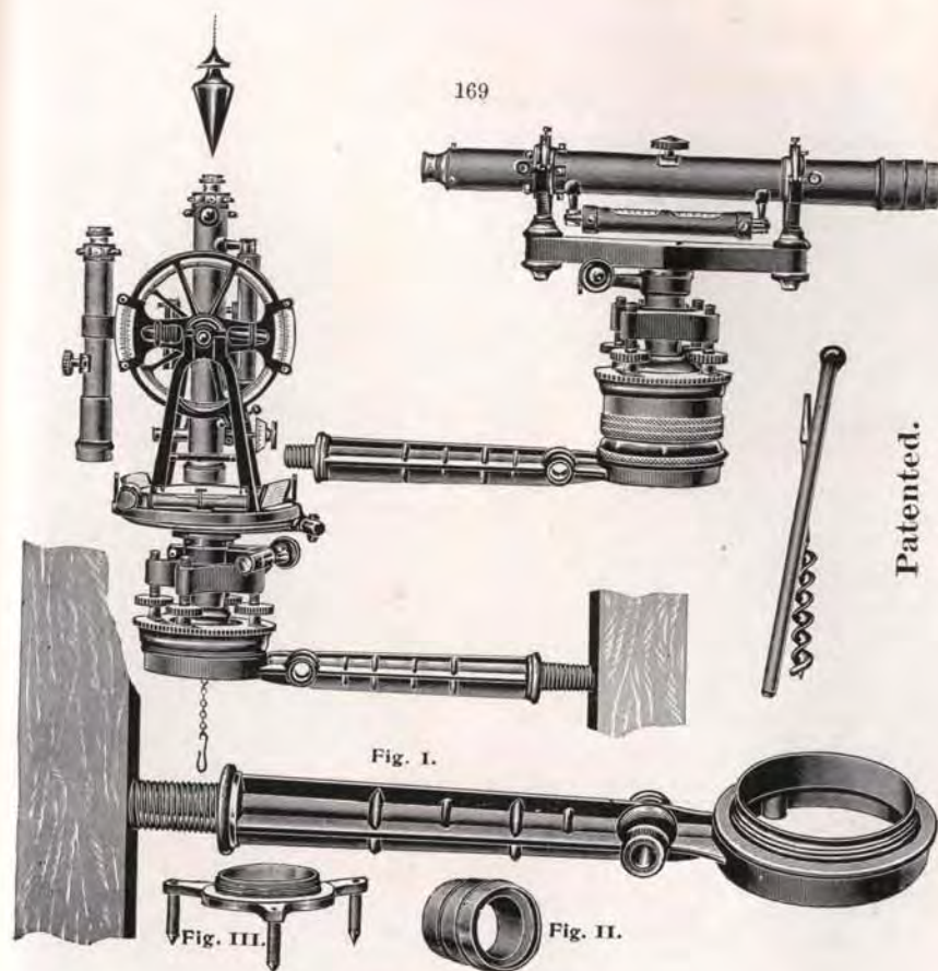
C. L. Berger & Sons' Bracket for Transit or Level.
