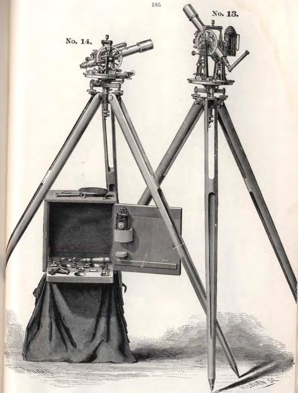
Astronomical Transit-Theodolite.
