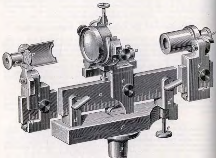
The Focal Length Apparatus.
