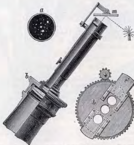
The Collimator used for testing Objectives of larger Telescopes.
