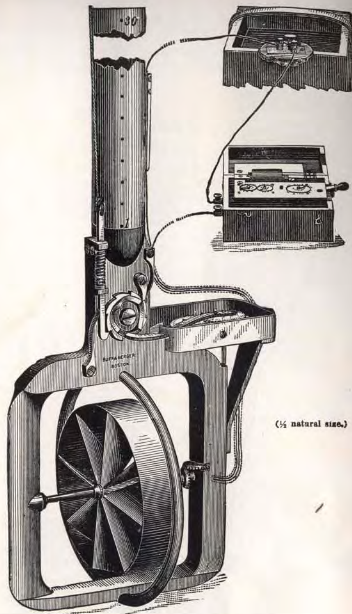
Current Meters No. V and VI.
