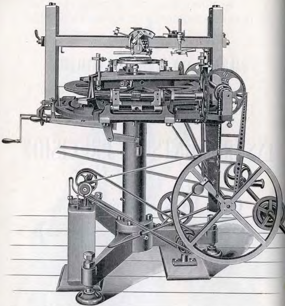
C. L. Berger & Sons' 30" Automatic Dividing Engine.
