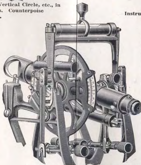
Instrument with Striding Level attached.
