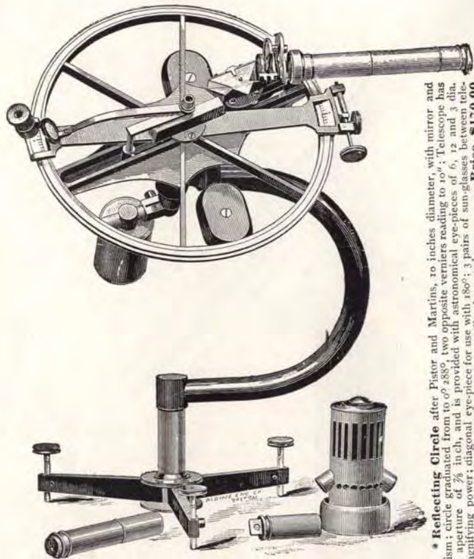
Reflecting Circle.*
