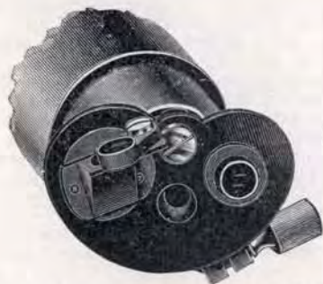
C. L. Berger &amp; Sons' Improved Prism and Colored Glass Attachment for Solar Observations.
