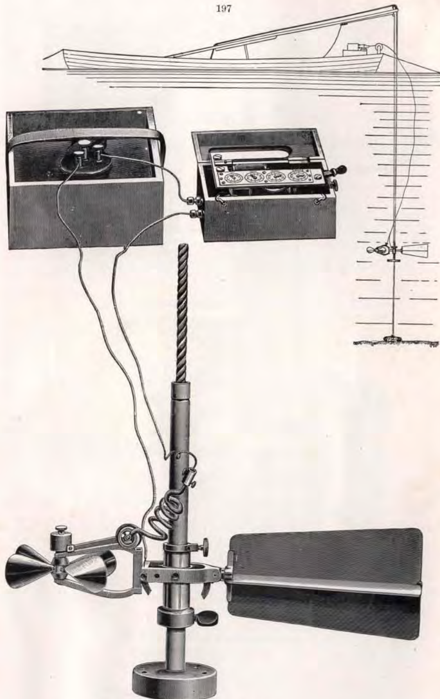
Current Meter No. IV.
